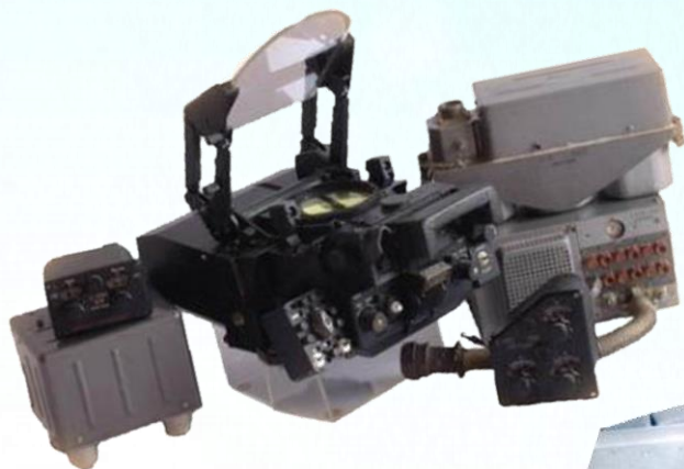
Sighting system
